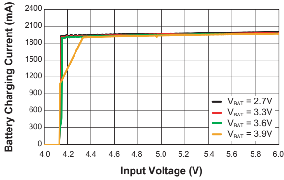
Charge Current vs. Input Voltage (T = -25°C)
