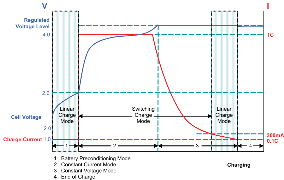
Figure 1: Current vs. Voltage and Charger Time Profile.
