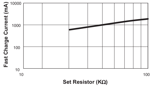
Current vs. I SET Resistor (V IN = 5V; V BAT = 3.5V)
